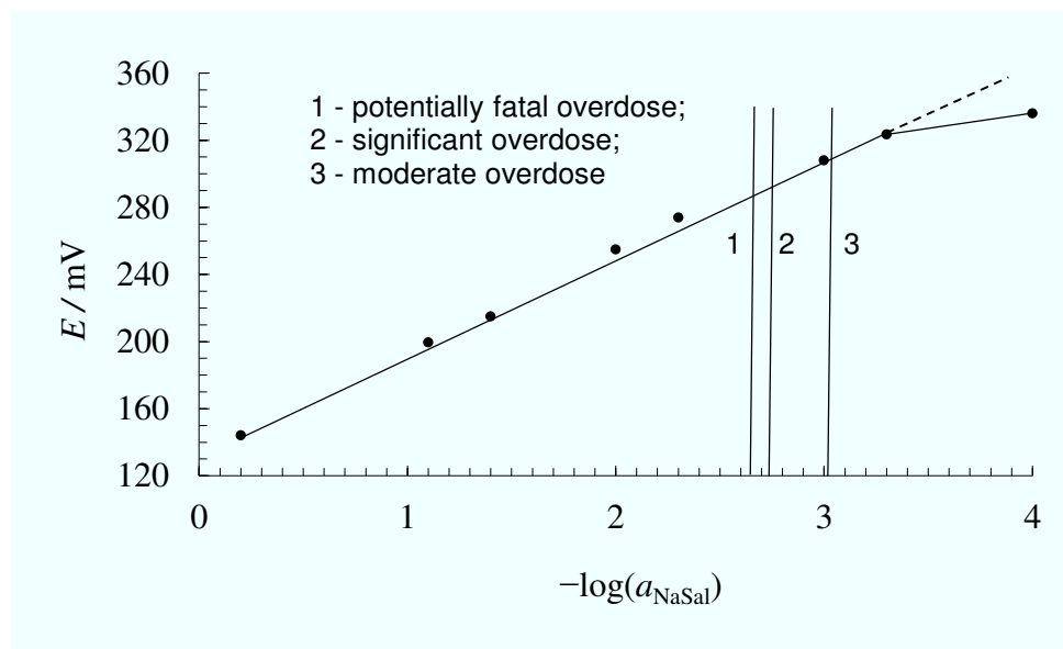
Fig. 5 Potentials of type I solid-state electrodes in NaSal +NaCl (0.12 M) solutions at pH 5.3
