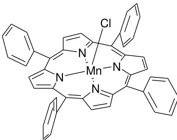
Fig. 1 Manganese tetraphenylporphyrin chloride ( \text{Mn(III)TPPCl} )
